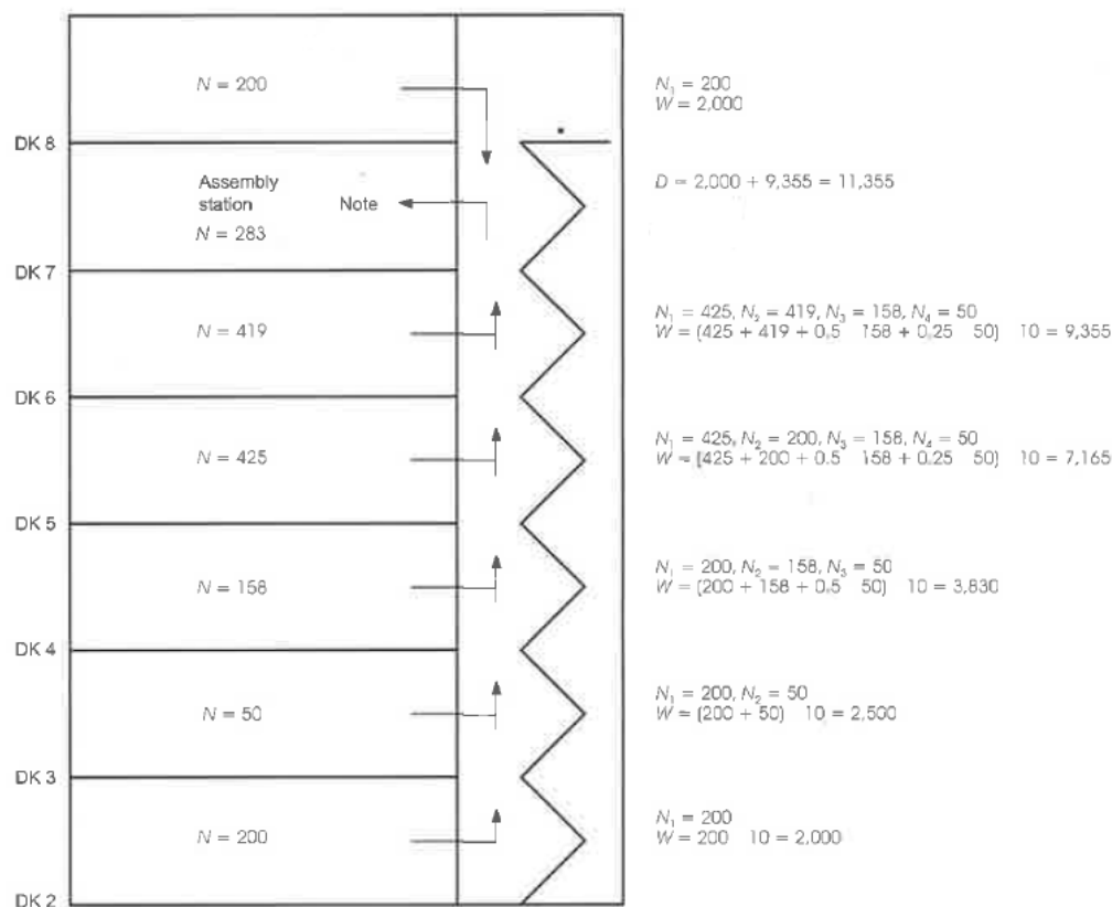
Figure 2 - Minimum stairway width ( W ) calculation example
