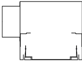
Headbox Section (motor on LH)
