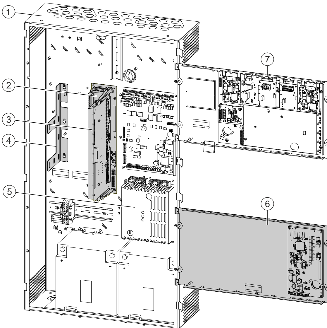
Fig. 2: FC724-ZA with extinguishing card and one extinguishing terminal
