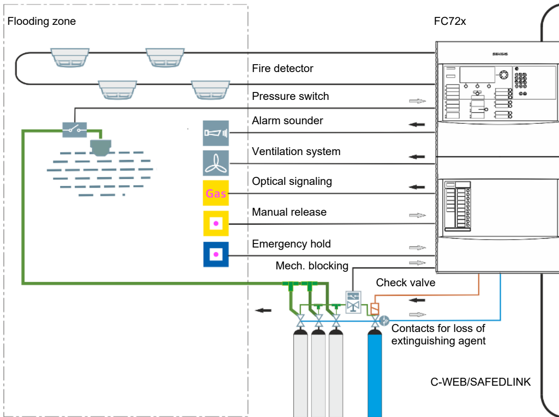
Fig. 1: Example: Single-sector extinguishing with monitoring and control from one fire control panel
