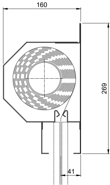
Headbox Detail
